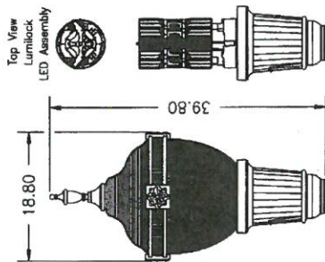
Luminaire Detail Scale 1:16
