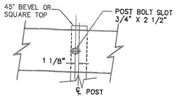
STEEL POST CONNECTION N.T.S.
